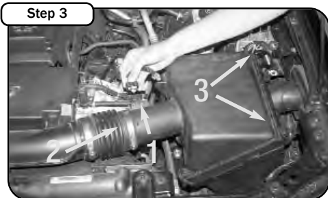
Step 3 Disconnect the MAF sensor (1). Loosen the hose clamp on the air box (2), and unclip the upper portion of the air box (3).
