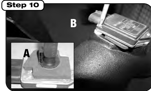
Step 10 Using provided gasket (A), slide onto mass air sensor. Using provided #6-32 screws and plastic spacers to mount mass air sensor onto tube (B). Once tight reconnect electrical terminal to sensor. Also replace filter minder and reconnect the electrical terminal.
