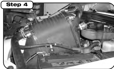
Step 4 Remove complete stock intake assembly from vehicle, including the factory accordion coupler.
