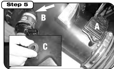
Step 5 If equipped with MAF sensor, remove MAF sensor (A) using provided T20 tork bit. Remove filter minder and factory grommet (B) from factory intake track. Install rubber grommet (C) into 3/4" hole in tube. Do not install filter minder yet.
