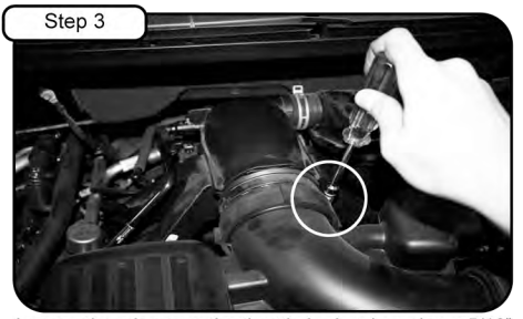
Step 3 Loosen the clamp on the throttle body tube using a 5/16" nut driver.
