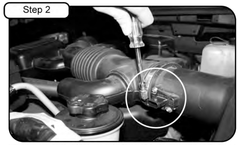
Step 2 Disconnect the MAF sensor harness. Loosen the clamp on the airbox tube using a 5/16" nut driver.
