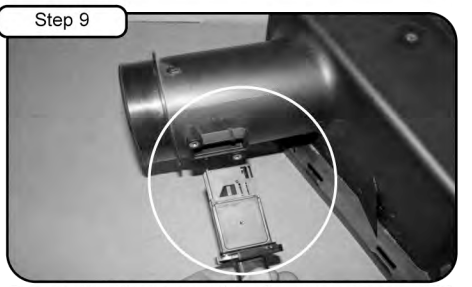
Step 9 Remove the MAF sensor from the airbox using a T-20 torx bit and save hardware for later install.
