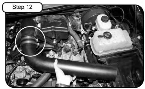
Step 12 Attach the intake tube to the vehicle with the straight coupler and clamps provided. Do not tighten clamps.
