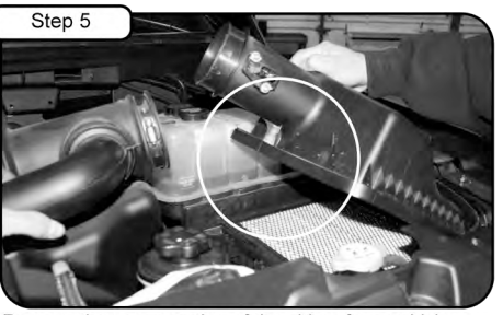
Step 5 Remove the upper portion of the airbox from vehicle.
