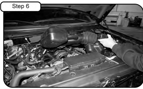
Step 6 Remove the stock intake tube from the vehicle.
