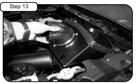
Step 13 Install the new housing into vehicle. Engage the clips, secure housing and connect the intake tube to coupler.
