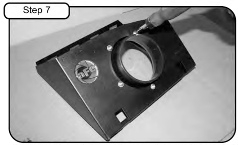
Step 7 Attach the filter adaptor to the new housing using button head screws provided and tighten using a 4mm allen key.
