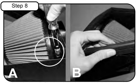
Step 8 A) Attach the air filter to the adaptor and tighten using a 5/16" nut driver. B) Attach trim seal to housing.
