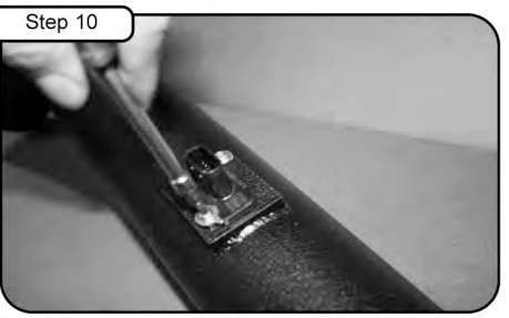
Step 10 Install the MAF sensor into the new tube using the screws removed in step 9.
