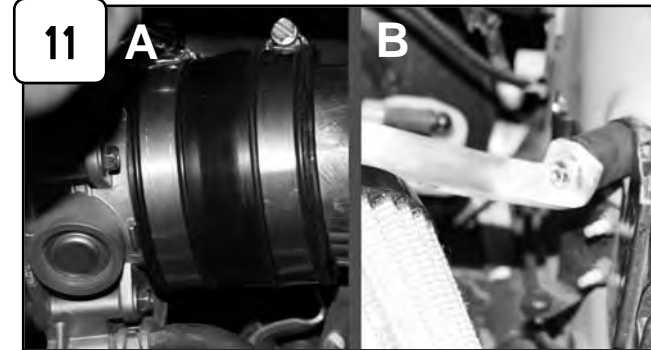
11 A) Install into vehicle and position coupler to throttle body and tab to isolation mount. B) Secure tab using flat washer, wavy washer and nut provided. Tighten using 10mm socket or wrench. Tighten clamps using 5/16" nut driver.
