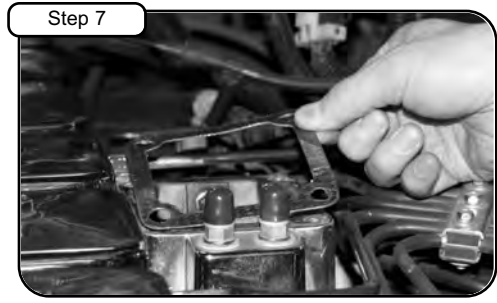
Step 7 Remove both top and bottom stock gaskets away from air grid heater. Replace with new gaskets provided. (May require a scraper or scotch brite to clean sealing surfaces.)
