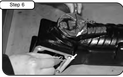
Step 6 Insert the 2 shorter M8 socket cap screws through aFe manifold. Hold washer against inside mounting flange of aFe manifold and feed screw completely through. Insert the two longer M8 screws w/ washers through the outside mounting bosses.
