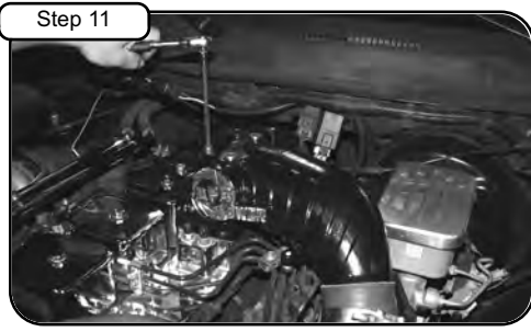
Step 11 With 6mm hexagonal bit provided and 6mm socket, install the four mounting bolts. Do not tighten completely! Use hex flange head screw provided and install on intake plate. Torque screw to 18 ft. lbs..
