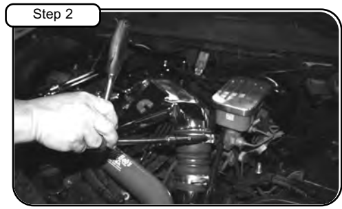
Step 2 Use 7/16" deep socket with ratchet to loosen the intercooler coupler hose clamp. Remove the screw holding engine oil dipstick.
