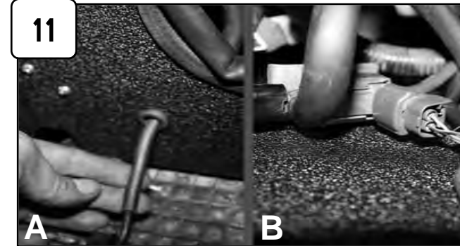
11 A) Install grommet to hole in housing. Run vacuum line through grommet. B) Re-connect sensor harness.
