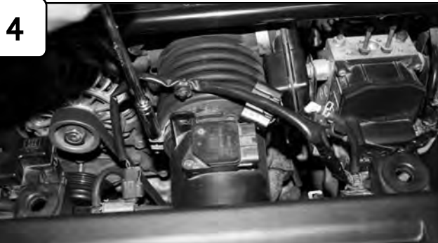
With 10mm socket or wrench loosen clamp holding in air box.
