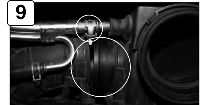
Loosen the clamp holding the lower intake box to the intake tube, then with pliers remove the pressure clamp holding the crank case breather line.
