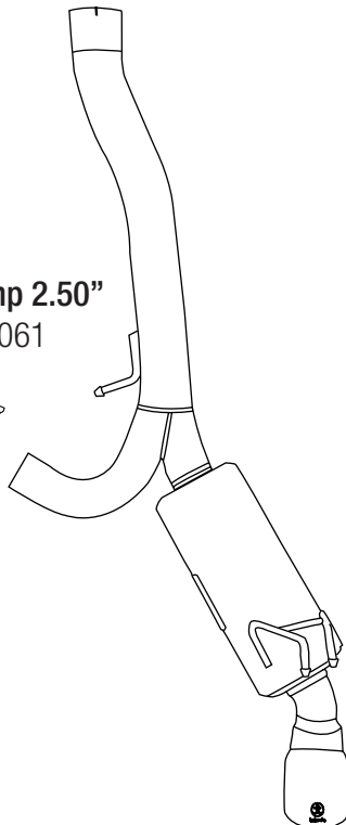
Right Side Muffler Section 05-45680 (Polished tips) 05-45680B (Black tips) 05-45680L (Blue flame tips)
