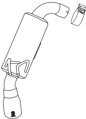
Left Side Muffler Section 05-45677 (Polished tips) 05-45677B (Black tips) 05-45677L (Blue flame tips)
