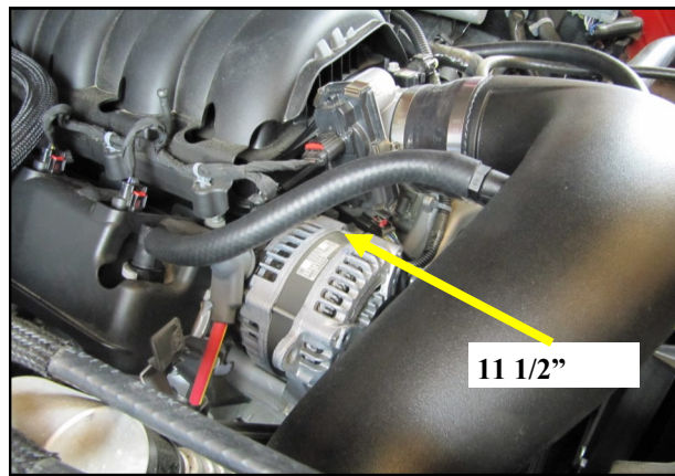
11. The 11 1/2" Hose is to be used on the Passenger side as shown.
