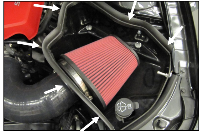
18. Install the Airaid Premium Filter (#1) onto the filter adapter and tighten the clamp. Next install the weather strip onto the top of the CAB. For ease of installation, start the front of the CAB near the radiator and work your way around towards the fender. Re connect the negative battery cable.
