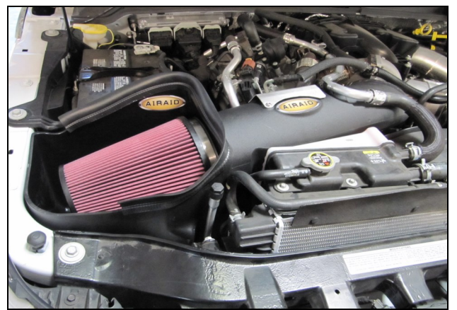
18. Install the Airaid Premium Filter (#1) inside the CAB and complete the install by trimming the CAB with the Weather Strip (#6).
