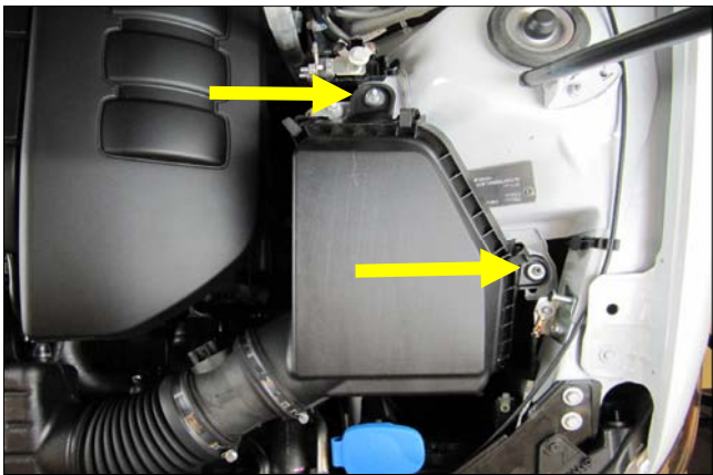
3. Remove the two 6mm flange nuts securing the air box assembly to the inner fender.
