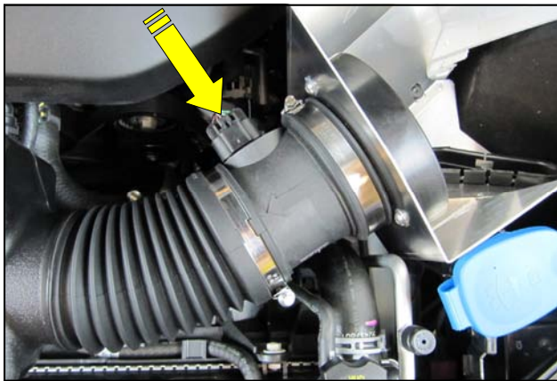
13. Check the positioning of the Mass Air Flow meter in relation to the wire harness. Readjust if necessary and tighten the clamps. Reconnect the Air Flow meter.
