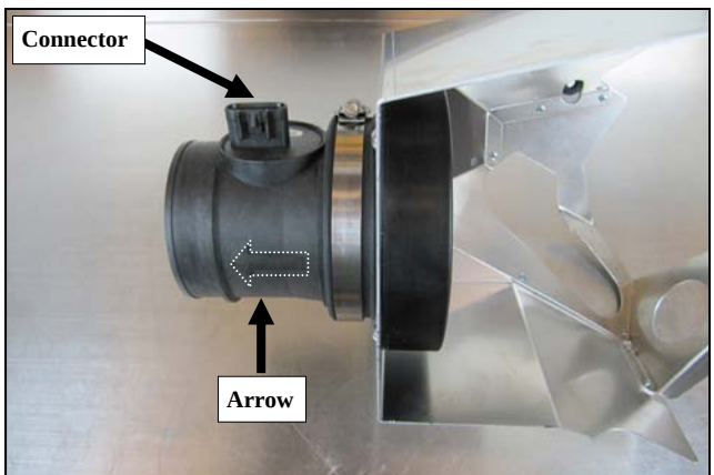
9. Transfer the Mass Air Flow meter into the Coupler as shown. Note the location of the connector and direction indicating arrow. Do not tighten the Clamp at this time.
