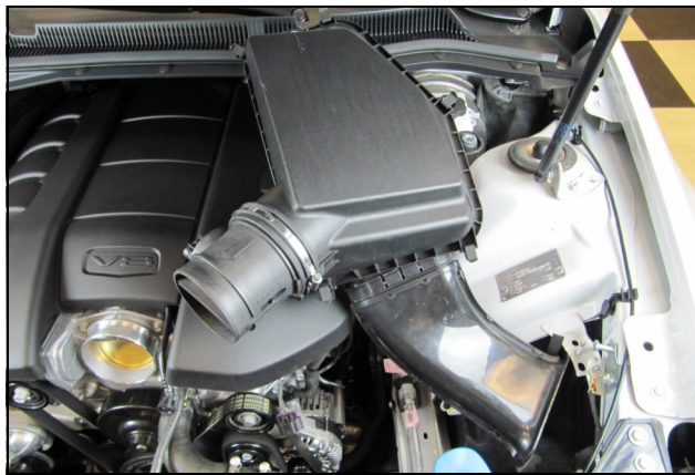
4. Remove the entire air box assembly from the vehicle.
