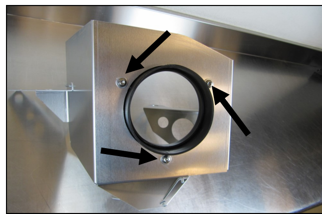
6. Install the Filter Adapter onto the Air Dam as shown using the three Button Head Screws and Flat washers.
