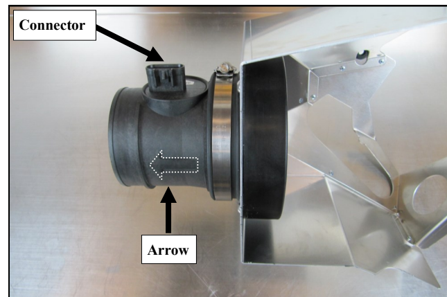
9. Transfer the Air Flow meter into the Coupler as shown. Note the location of the connector and direction indicating arrow. Do not tighten the Clamp at this time.
