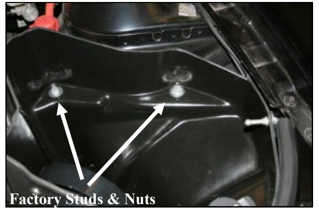
12. Install the Airaid Cold Air Box into the vehicle locating the factory grommets over the factory studs. Re-install the factory nuts from step #3 onto the studs. Reinstall the factory ground lug thru the Airbox wall.
