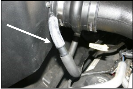
14. 2004-07 Models; Reconnect the factory breather hose to the 1/2" barbed fitting on the CAD using the 1/2" rubber elbow (#13), and 1/2"x 3/4" barbed fitting as shown.
