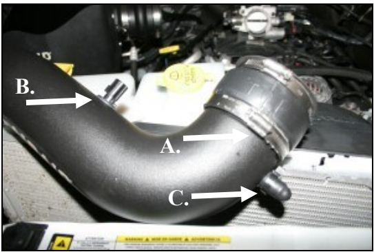
12. A.) Reinstall the factory coupler and hose clamps on to the Airaid intake tube (#2). Tighten the hose clamp on the tube. 2003-07 Models; B.) Install the supplied grommet (#11) into the hole in the Airaid tube, and then carefully push the factory air temperature sensor into the grommet. 2002 Models; Install the grommet plug (#10) in place of the grommet. 2004-07 Models; C.) Slide the rubber cap (#12) over the nipple on the Airaid intake tube and secure it with the #14 speed clamp (#14).
