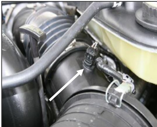
5. STOP AND LOOK! If you have a temperature sensor like this, disconnect the temperature sensor wiring harness, remove the sensor from the tube (save it for reuse) and proceed to step #8. The early production 2005 F-250 and F-350 6.0 diesel trucks either came with a temperature sensor, or they came with a Mass Air Flow (MAF) sensor. These pictures will help you determine which sensor you have. Whichever sensor you have, this Airaid Intake System will fit .
