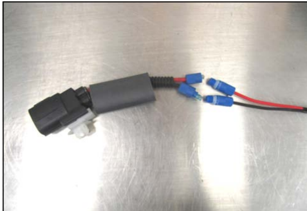
24. Slide the large heat shrink tubing on to the wiring harness. Hand tighten the threaded female cap and wire into the Posi Lock® connector.
