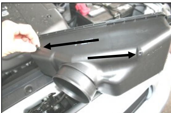
8. Install the two rubber washers (#19) onto the two plastic plugs (#18) that are provided in the hardware kit, and insert them into the two weep holes in the factory air cleaner cover removed in step #4, as shown
