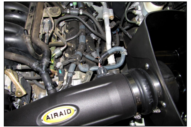
12. Reconnect the factory PCV breathers and spring clamps to the Barbed "Y" Fitting. Reconnect the Mass Air Flow sensor.
