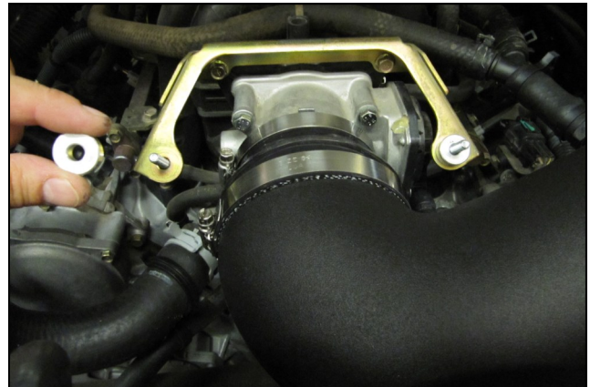
15. Reinstall the bracket onto the intake manifold and place a Spacer (#13) onto each 6mm bolt.
