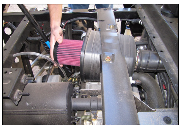
20. Tilt the bed back and install the Airaid Premium filter (#1).
