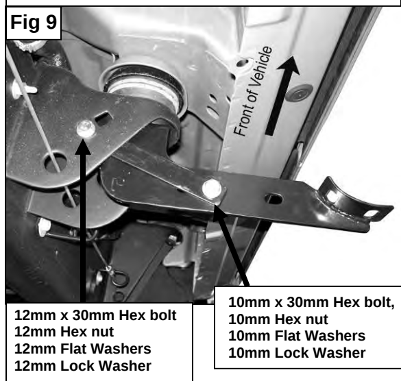
99-10 2500 Model Center Installation Pictured
