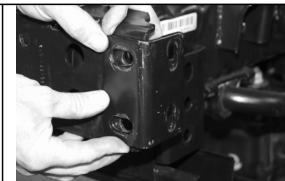
Fig 2 Note the orientation of the bolt holes
