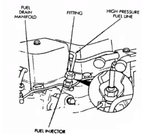
Fig 10: Fuel Lines at Fuel Injectors
