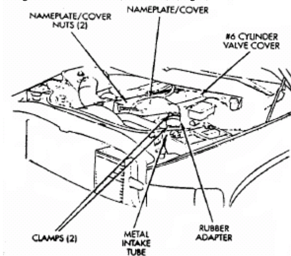
Fig 9: Nameplate/Cover - Diesel
