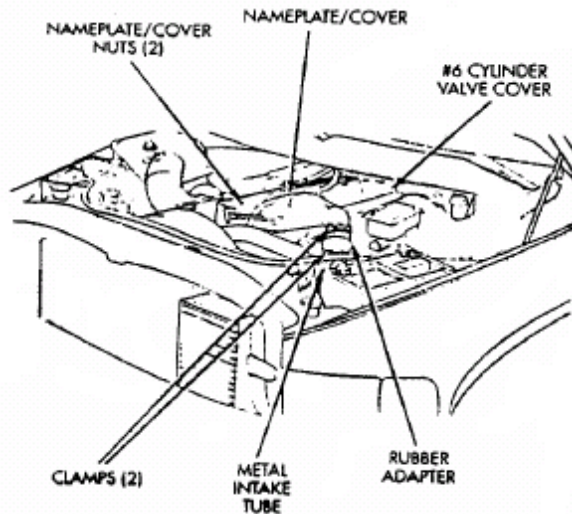
Fig 9: Nameplate/Cover - Diesel
