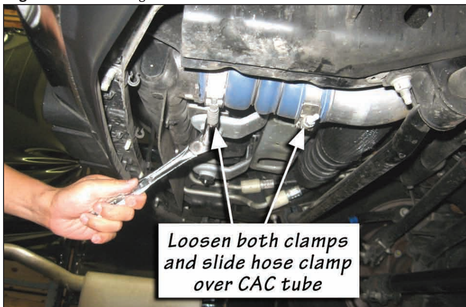
Figure 3 Disconnecting the Driver Side CAC Tube
