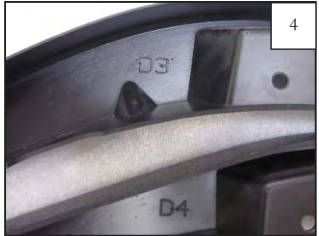
Locate the flat flare rear inner pieces. The driver side rear inner pieces are marked D3 & D4. The passenger side rear inner pieces are marked P3 & P4.
