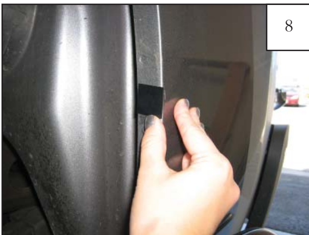
Center a supplied Black Plastic Tab over the remaining four marks made in Step 4, aligning edge of tab with inside of fender lip (tab may extend over outside of fender).
