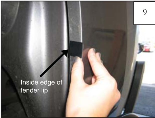
Center a supplied Tab (MT1-0002) over the marks made in step 7, aligning edge of tab with inside edge of fender lip (tab may extend over outside of fender).
