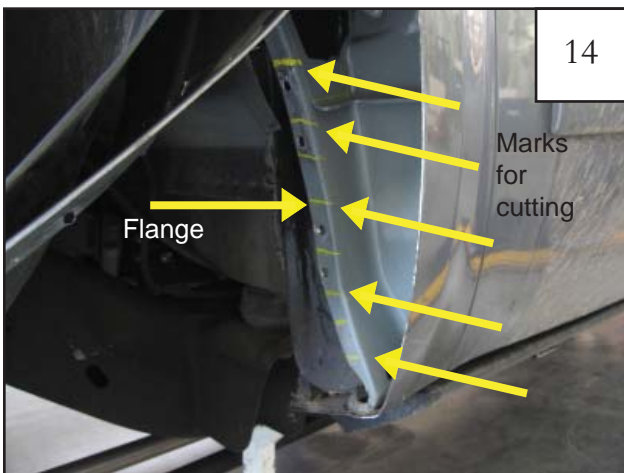
Mark the flange on the inner fender support structure approximately every 2". NOTE: Horizontal marks will be cut to create metal tabs.
