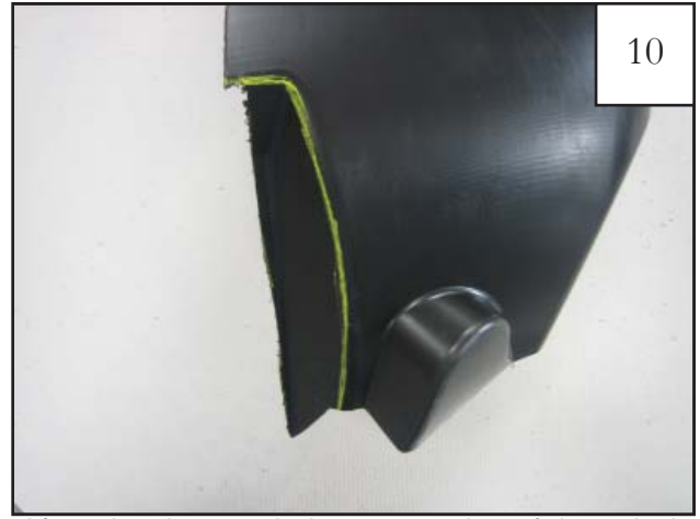
After trimming, mark the rear portion of the splash shield as shown and trim. NOTE: If trimmed too little, flare won't fit; if trimmed too much, shield won't stay behind flare.
