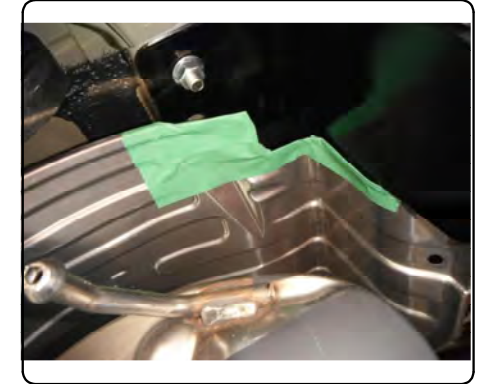
HEAT SHIELD TRIMMING DIAGRAM NOTE: TRIM DIMENSIONS ARE APPROXIMATE, CONFIRM FIT PRIOR TO TRIMMING.
