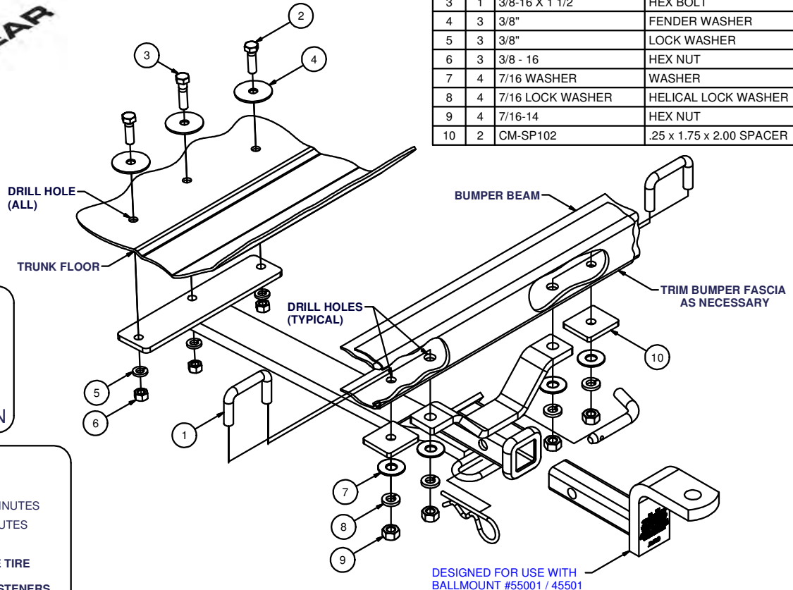
U-BOLT INSTALLATION
