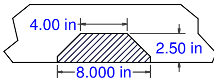
EDGE SPORT FASCIA TRIM DIAGRAM
