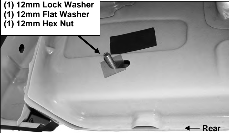
(Fig 6) Rear mounting position pictured
