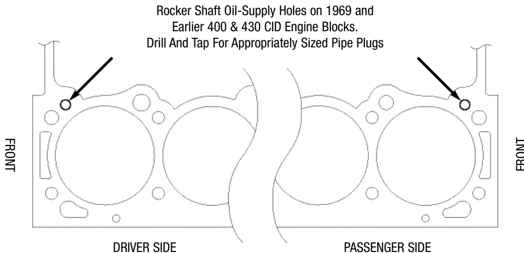
TYPICAL DECK VIEW OF 1969 AND EARLIER BUICK ENGINE BLOCK
