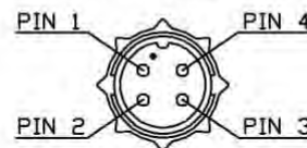
PIN VIEW
