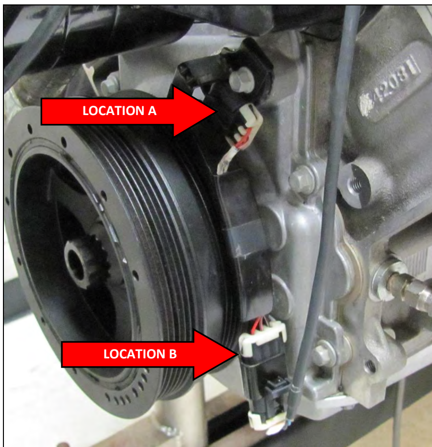
Proper Holley Harness Connection Location
