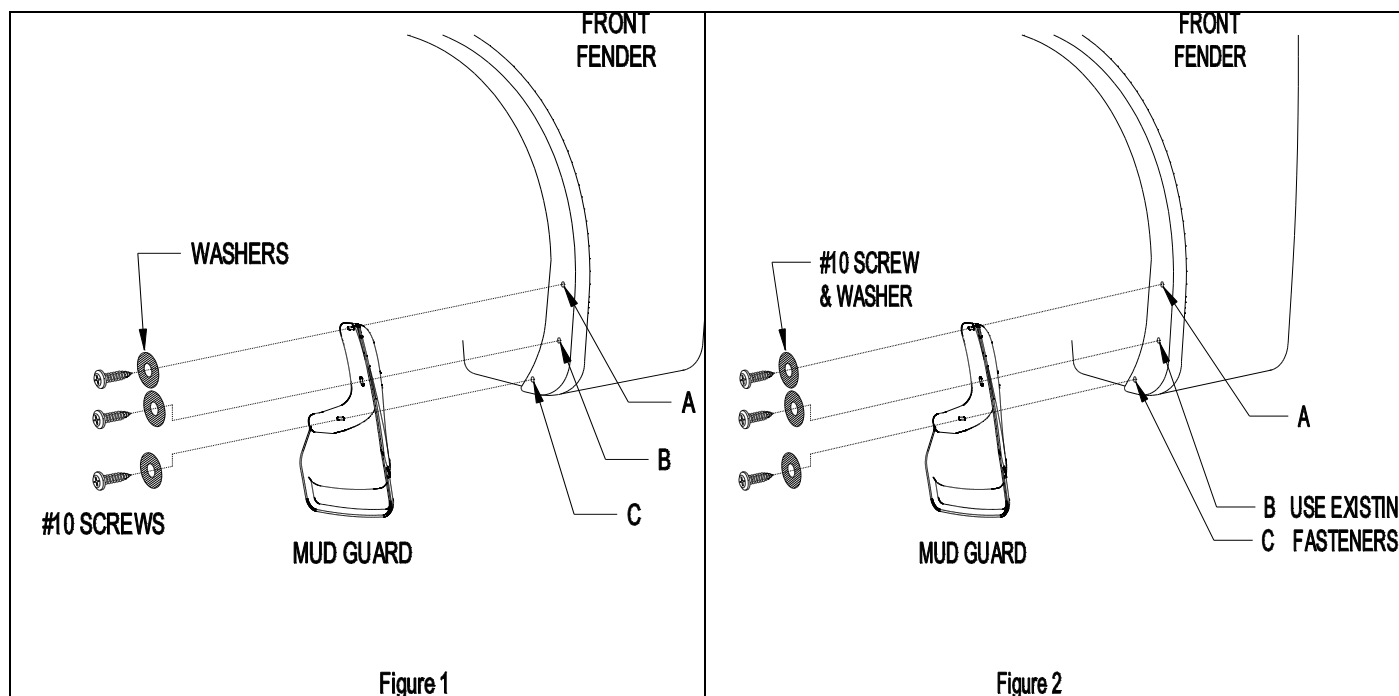
Figure 1 F-150 with flares
