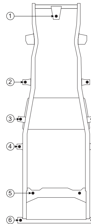
BODY MOUNT LOCATION DIAGRAM
