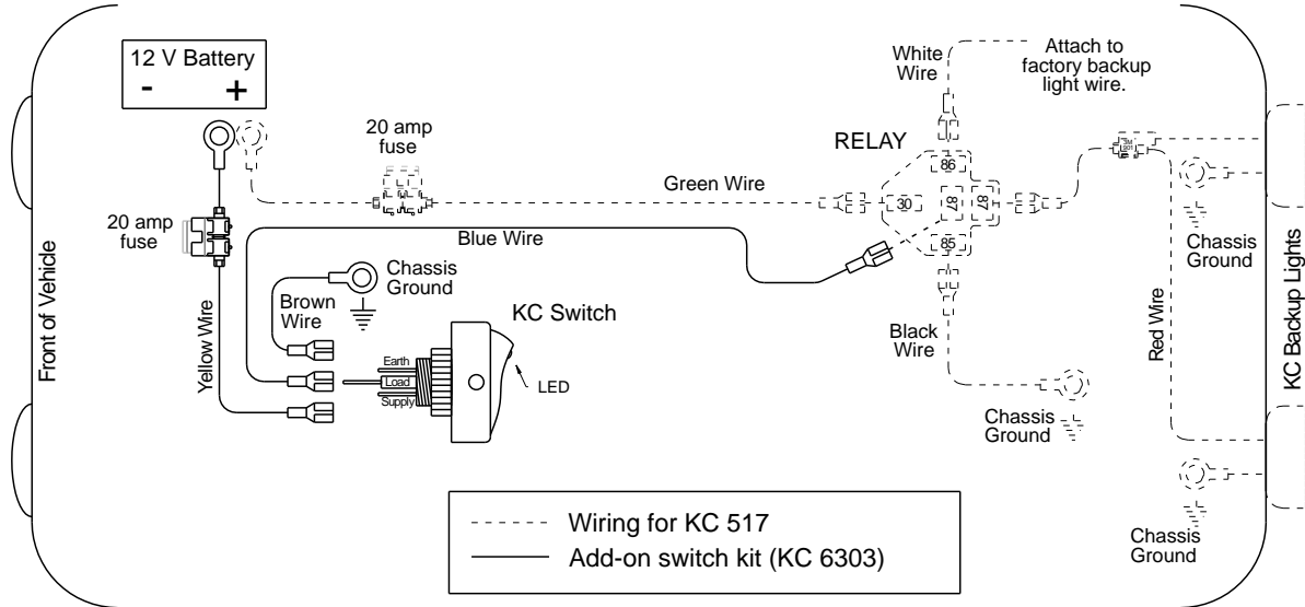
Diagram for Optional KC 6303 Add-On Switch Kit
