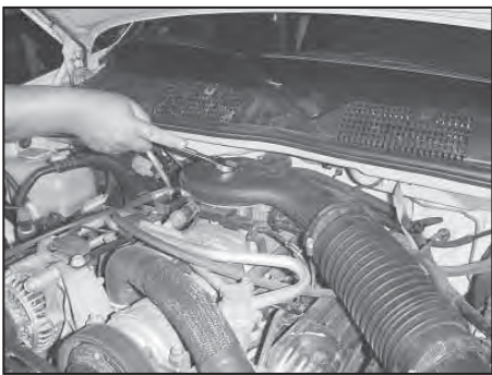
2. Loosen the nut at the intake plenum as shown.
