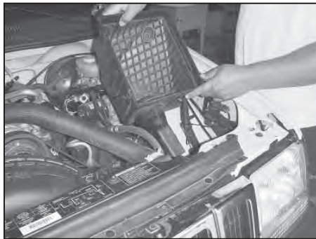
6. Remove the airbox base as shown. NOTE: K&N Engineering, Inc., recommends that customers do not discard factory air intake.
