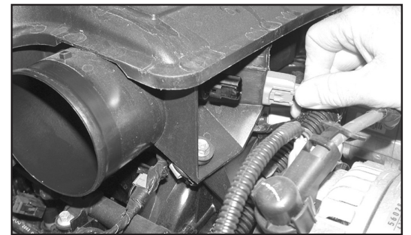
7. Depress the locking tab on the air temp sensor and disconnect its electrical connection.
