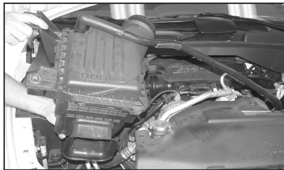
5. Pull up firmly to dislodge the air box from the mounting grommet, and remove the air box from the vehicle.
