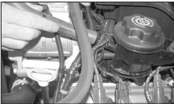
2. Disconnect the crank case vent hose at the oil filler stand off as shown.
