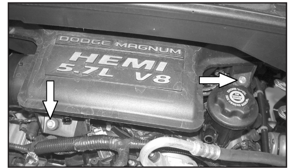
8. Remove the two 10mm resonator retaining bolts, then remove the resonator from the vehicle. NOTE: K&N Engineering, Inc., recommends that customers do not discard factory air intake.
