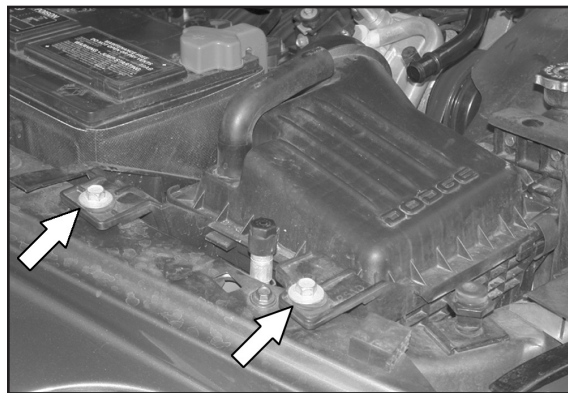
4. Remove the two airbox retaining bolts.
