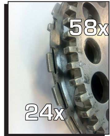
Figure 16 Crank Shaft Reluctors.
