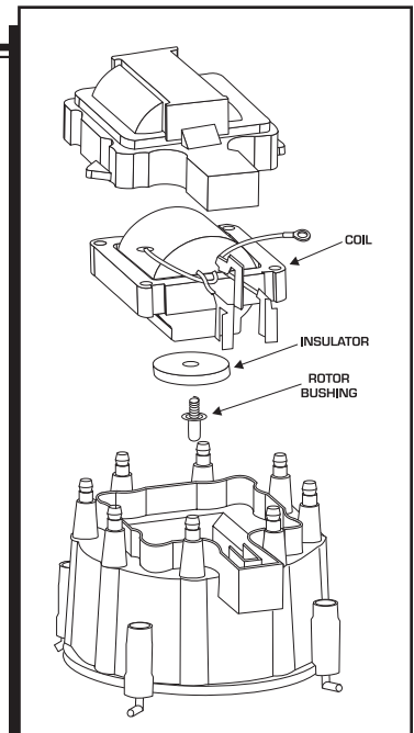
Figure 2 Installing the Street Fire GM HEI Coil.
