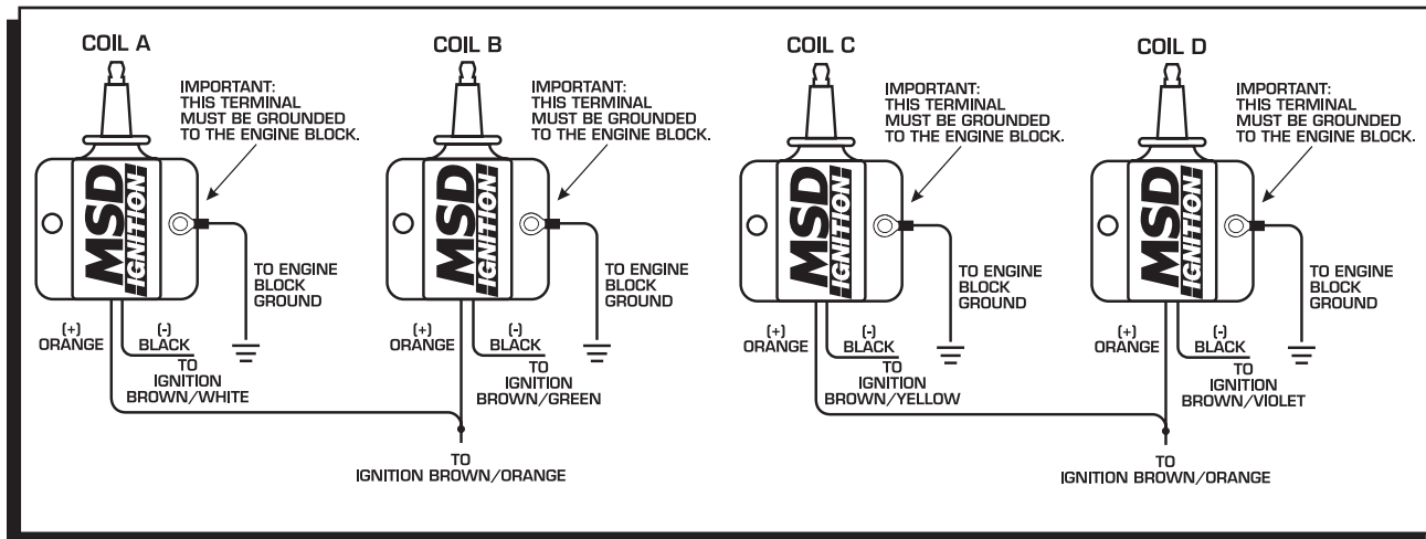
Figure 3 Four Coil System to DIS-4 Ignition.
