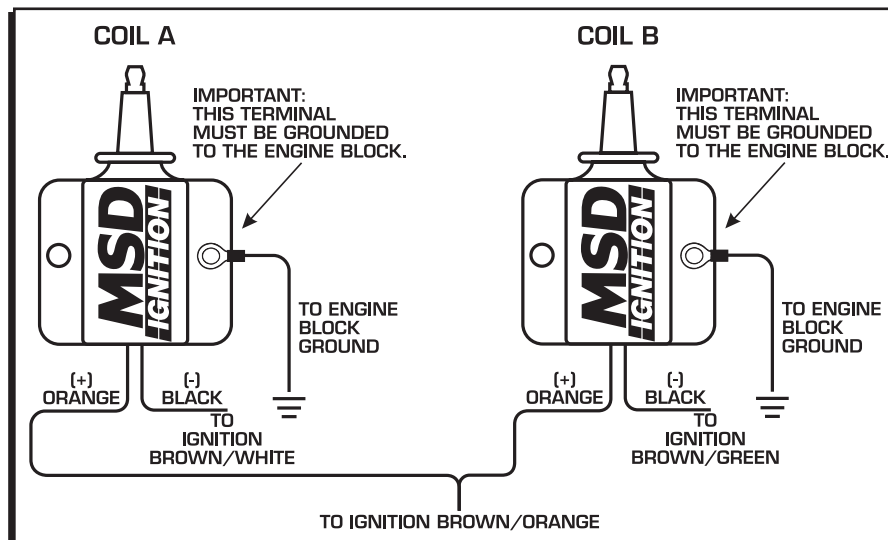
Figure 2 Dual Coil System to DIS-2 Ignition.
