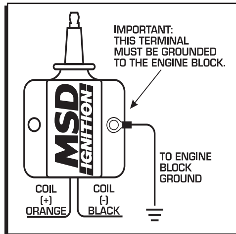
Figure 1 Grounding the Coil.
