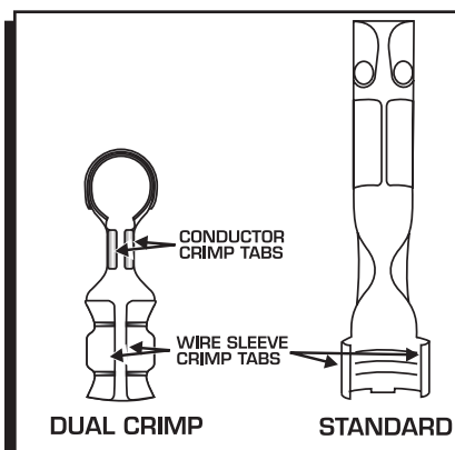
Figure 5 Identifying the Different Style Terminals.
