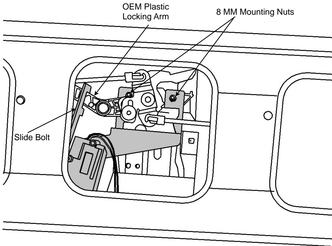
Diagram 2 - Assembled View
