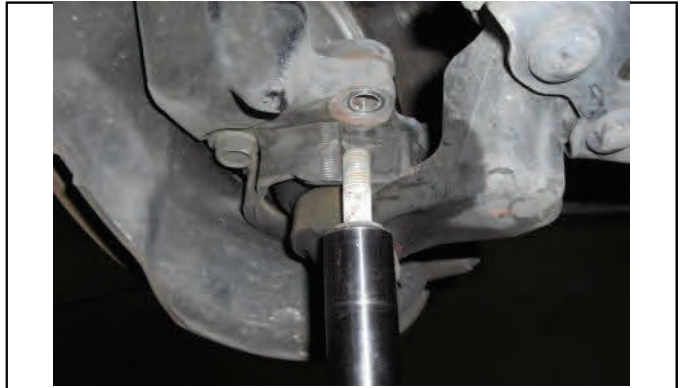
Disconnect lower ball joint hardware bolts
