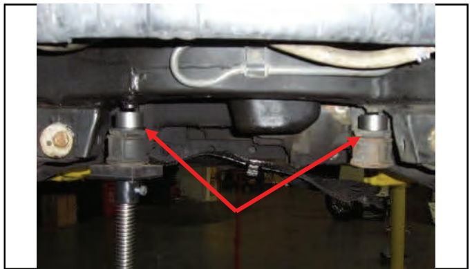
4WD Lower differential and place spacers as show
