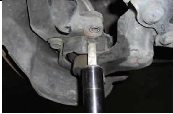
Disconnect lower ball joint hardware bolts
