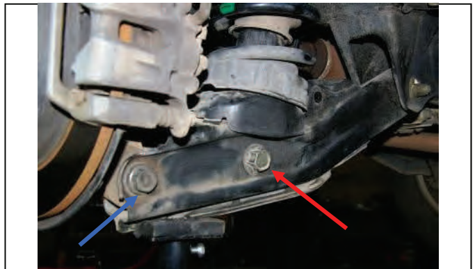
Reinstall lower strut bolt , raise arm and attach at spindle
